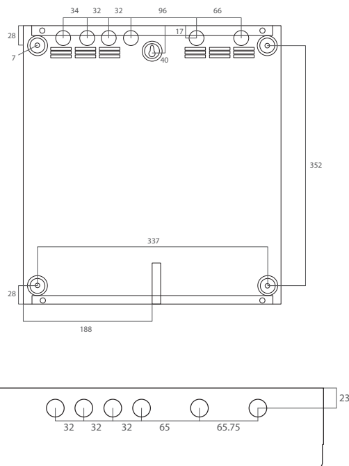
Rear of enclosure showing mounting holes
